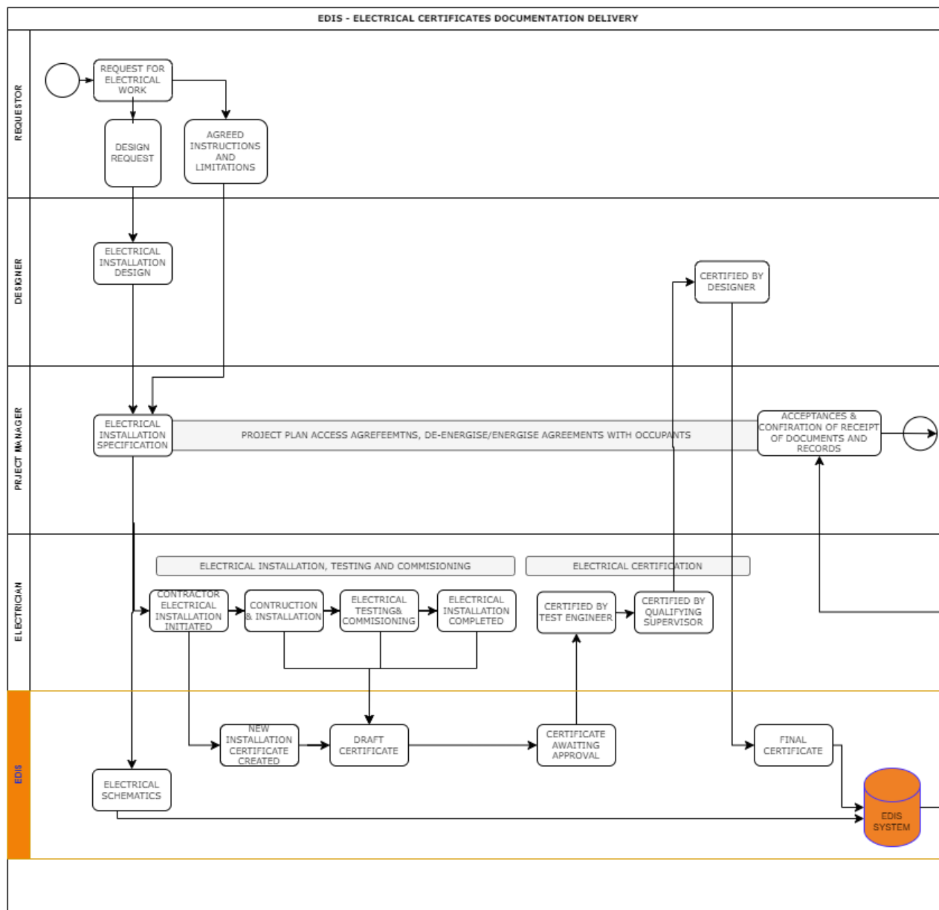
Figure 1- Process for delivering EDIS electrical certificates
