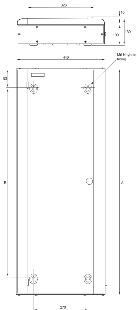
Split metered power and lighting board – 230A TPN, dimensional drawing
